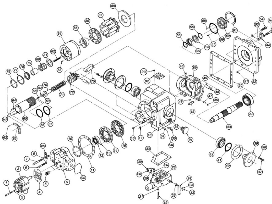
Variable Displacement Pump PV20
